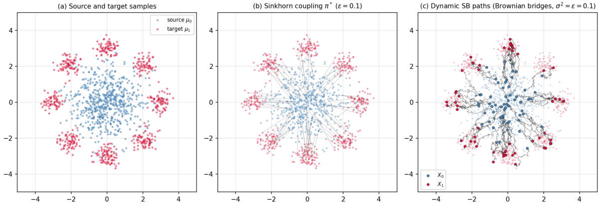
Figure 6.2.1: Schrödinger bridge between a 2D Gaussian source and an 8-mode ring target, computed by the Sinkhorn algorithm (6.2.10). (a) Source \mu_0 and target \mu_1 samples ( N = 600 each). (b) Optimal coupling \pi^* at regularization \varepsilon = 0.10 , visualized as line segments for 80 source–target pairs sampled from \pi^* . (c) Sample paths of the dynamic SB (6.2.5): for 60 pairs (X_0^*, X_1^*) drawn from \pi^* , the trajectory is a Brownian bridge with diffusion \sigma = \sqrt{\varepsilon} = \sqrt{0.10} between the two endpoints; circles mark X_0^* (blue) and X_1^* (red).
